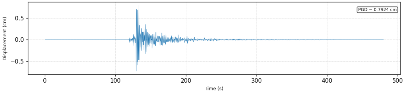
4. Ground Displacement
